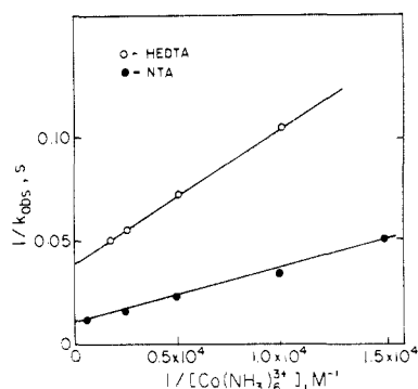
Figure 4. Reciprocal of k_{obs} of the decay of the complex with the metal-carbon \sigma -bond as a function of 1/[Co(NH_3)_6^{3+}] at pH 7 in N_2O -saturated solutions containing 6 mM L, 1 mM FeSO_4 , and 0.1 M formate: \bullet , L = NTA; \circ , L = HEDTA.
