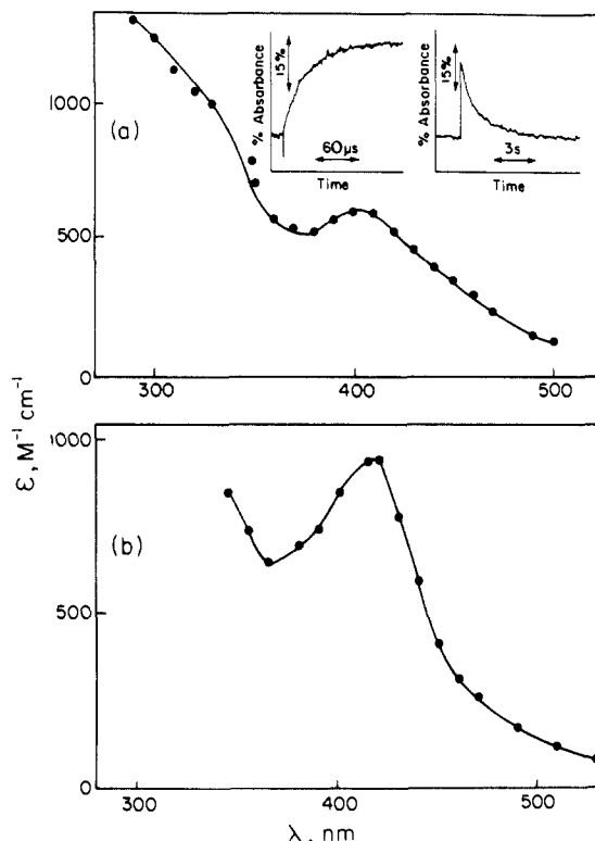
Figure 1. Transient spectra formed by the reaction of L-Fe^{II} with CO_2^- at pH 7 in N_2O -saturated solutions containing 0.1 M formate. The pulse duration was 0.5 \mu s and the optical path length 12.1 cm. Parts: (a) 6 mM NTA, 0.9 mM FeSO_4 ; (b) 3 mM HEDTA, 2 mM Fe(NH_4)_2(SO_4)_2 \cdot 6H_2O . The inset in (a) contains typical absorption traces of the formation and decomposition of the transient at 410 nm in N_2O -saturated solution at pH 7 containing 4 mM Fe^{II} , 6 mM NTA, and 0.1 M formate.
